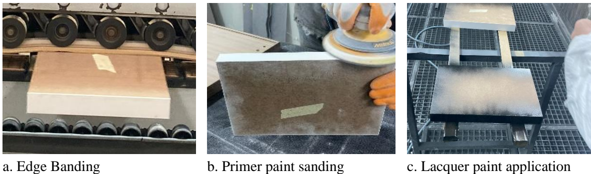
Figure 1. Preparation stages of test samples.
