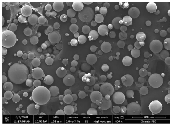
Figure 1. SEM image of hollow glass spheres (Kesik and Kabakcı, 2022).
