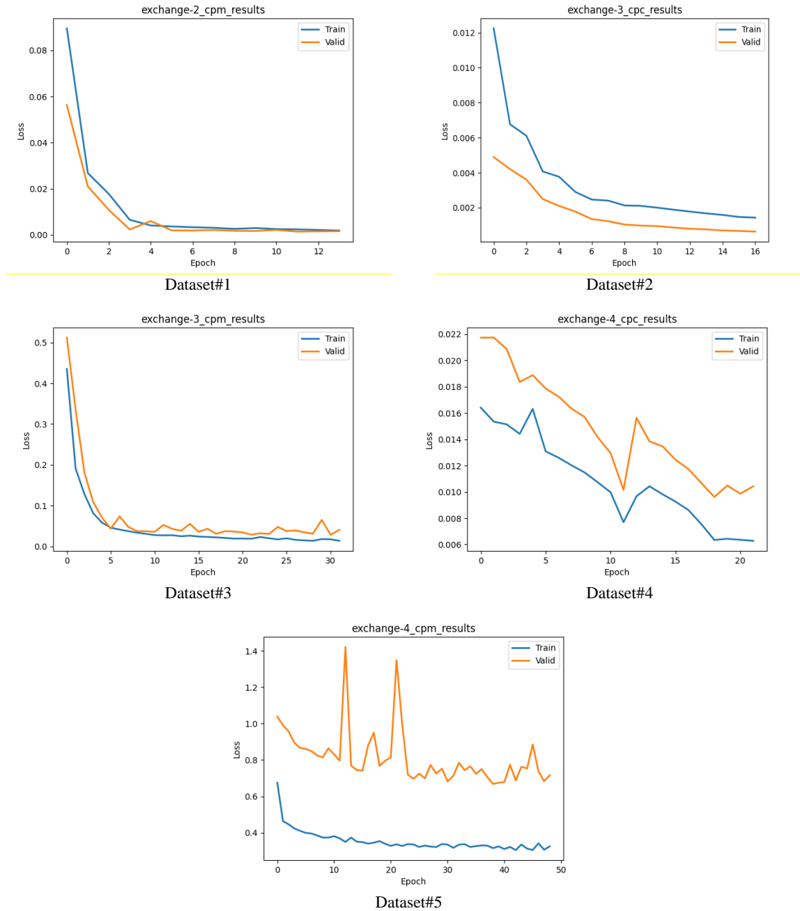
Figure 2. Training and validation loss curves of the LSTM-Ae model for each dataset.
